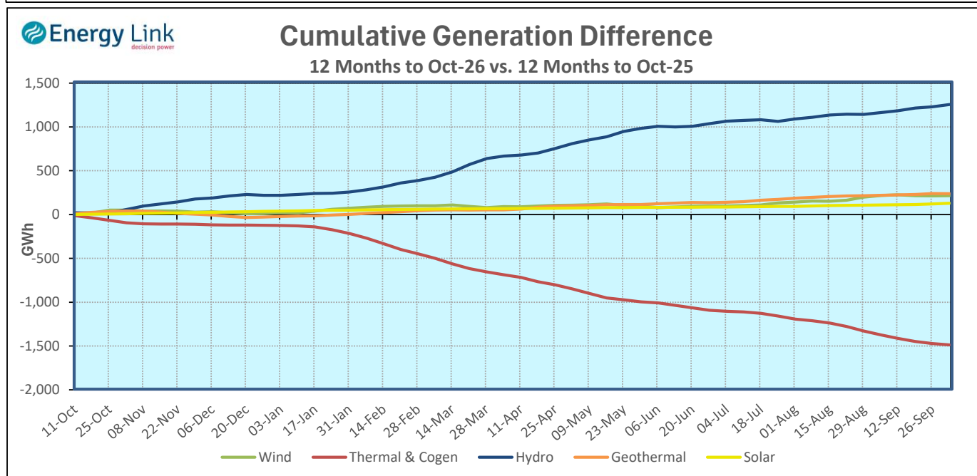
Cumulative Generation Difference, last 12 months vs. 12 months prior as of 04/10/2026
