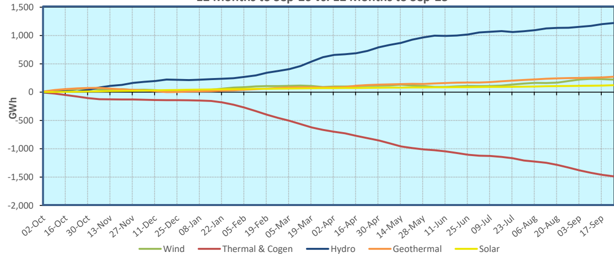
Cumulative Generation Difference, last 12 months vs. 12 months prior as of 25/09/2026
