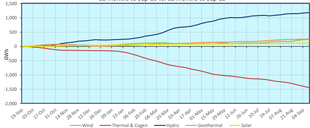
Cumulative Generation Difference, last 12 months vs. 12 months prior as of 12/09/2026
