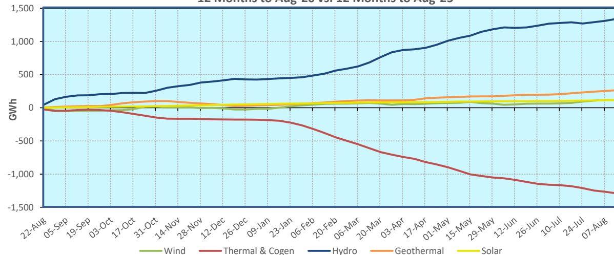
Cumulative Generation Difference, last 12 months vs. 12 months prior as of 15/08/2026
