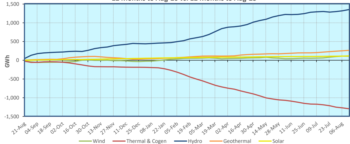
Cumulative Generation Difference, last 12 months vs. 12 months prior as of 14/08/2026
